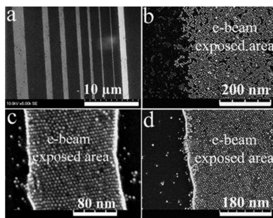
Figure 2. SEM images of ultrathin Au NP/PMMA films patterned with electron beam lithography. (a,b) Film patterned with lower e-beam dose and developed with hexane. (c, d) Film patterned with higher e-beam dose and developed with toluene plus 1-dodecane thiol (10:1 in volume).
